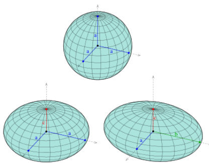
Figure 10.1: Ellipsoid 1
