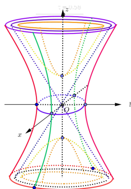
Figure 10.5: Hyperboloid and asymptotic cone 5
