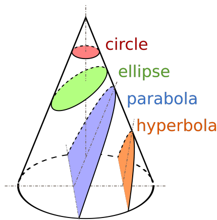
Figure 8.1: Conic sections 1
